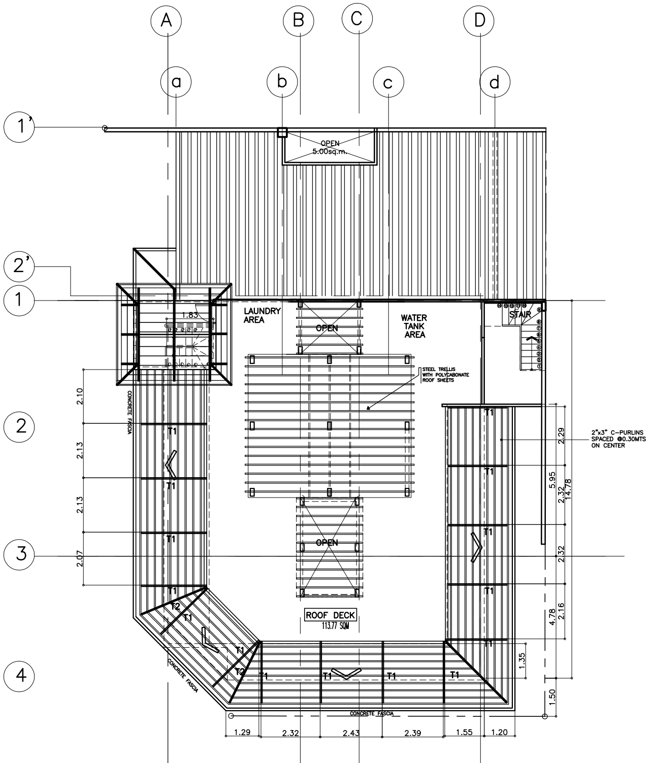
ROOF DECK PLAN SCALE 1:100M
