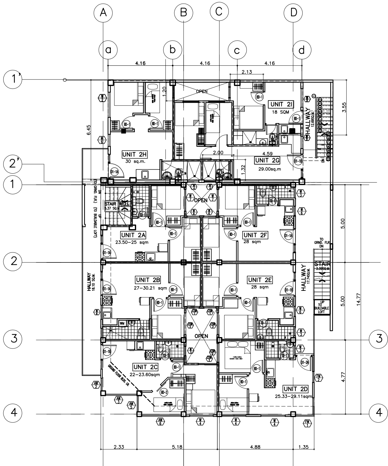
2 SECOND FLOOR PLAN A2 SCALE 1:100 mts
