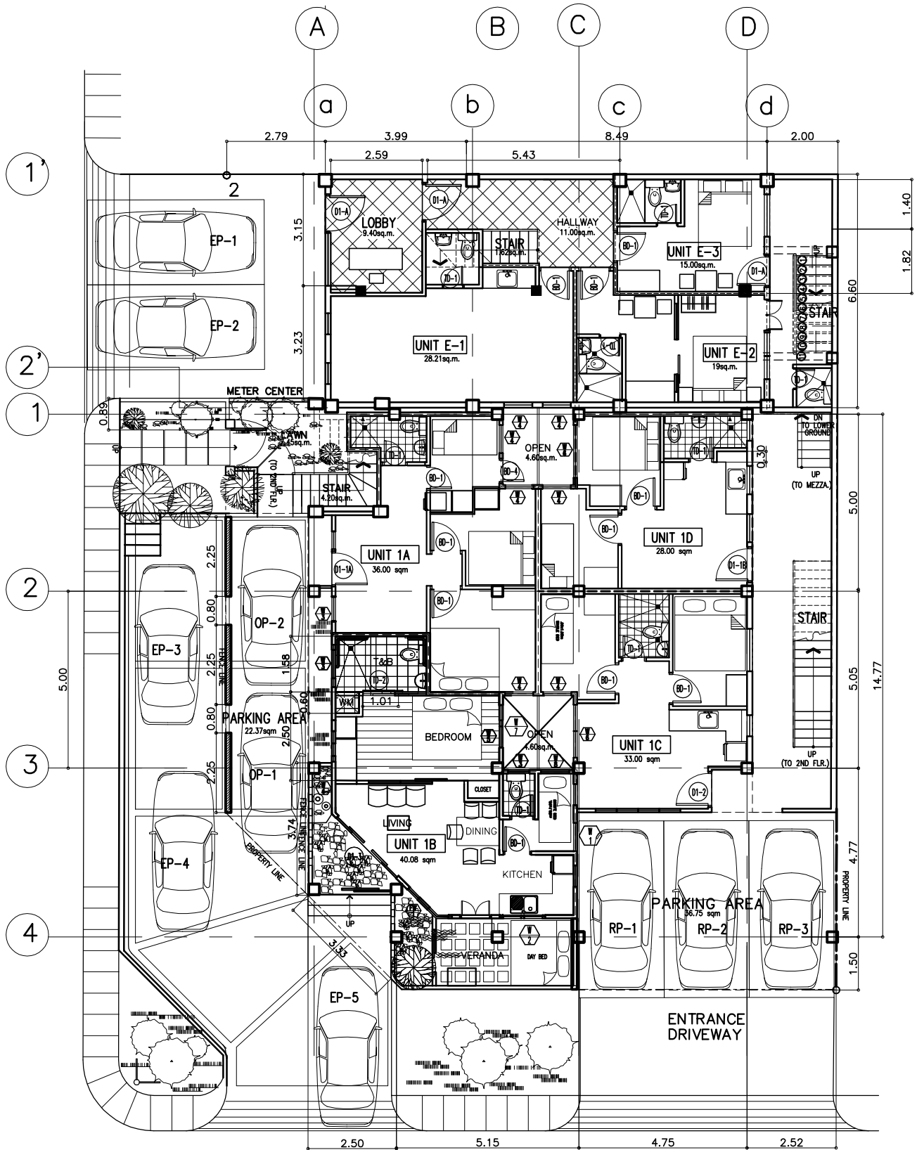
1 A2 GROUND FLOOR PLAN
